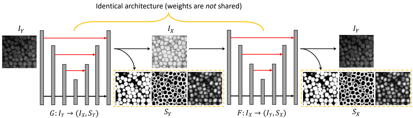
Fig. 2. Architecture details of CySGAN. Given an image sampled from I_Y , the generator G predicts both the transferred image in I_X and the BCD segmentation representations S_Y . Then the generator F takes only the translated image as input and predicts both the reconstructed image and segmentation representations. Specifically, BCD stands for “binary foreground mask,” “contour map,” and “distance transform map.” We visualize the predicted BCD representations in the dashed yellow boxes. The two generators have exactly the same architecture, but the weights are not shared as they are optimized to translate images in different domains. Only the generator G is needed to segment I_Y images at inference time (the output channel for translation can also be removed).
